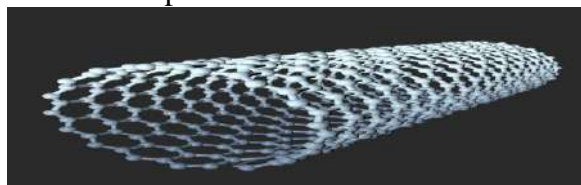
Figure 1: Carbon Nanotubes
