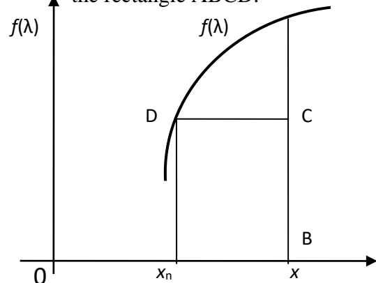
Figure 1.2 : Approximating the area by the rectangle ABCD. E
