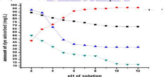
Fig 1: Effect of pH on the adsorption of the four selected dyes by ACT3 RED Curve: MeG, Black Curve: AY, Blue Curve: AY, Green Curve: MG
