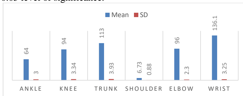
FIGURE 2: DESCRIPTIVE STATISTICS OF ANGULAR KINEMATIC VARIABLES OF SUCCESSFUL SHOTS DURING WIND-UP II
