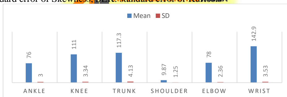
FIGURE 1: DESCRIPTIVE STATISTICS OF ANGULAR KINEMATIC VARIABLES OF SUCCESSFUL SHOTS DURING WIND-UP I
