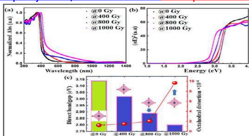
Figure 6. (a) UV-Vis absorption spectra for gamma-irradiated (dark line) and unirradiated (shaded lines) lanthanum zirconate (LZO) ceramics. (b) Tauc plot for the same materials, showing the relationship between absorption and energy. (c) Correlation between the bandgap and octahedral distortion in LZO ceramics.
