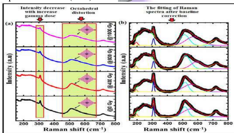
Figure 3. (a) Dark line: LZO ceramic Raman spectrum before gamma irradiation. (b) Fit post-irradiation Raman spectra for analysis.
