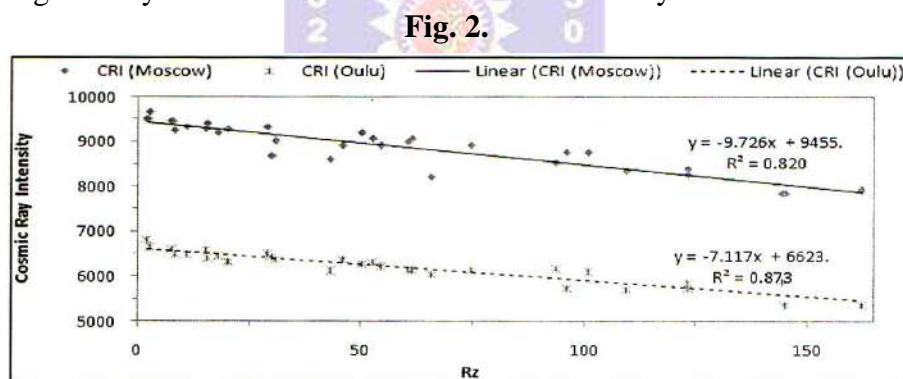
Fig. 2. Has show the linear correlation of yearly average vale of sunspot number with cosmic ray intensity (Moscow and Qulu) during period of solar cycle 22 to 24 from year 1992 to 2022.
